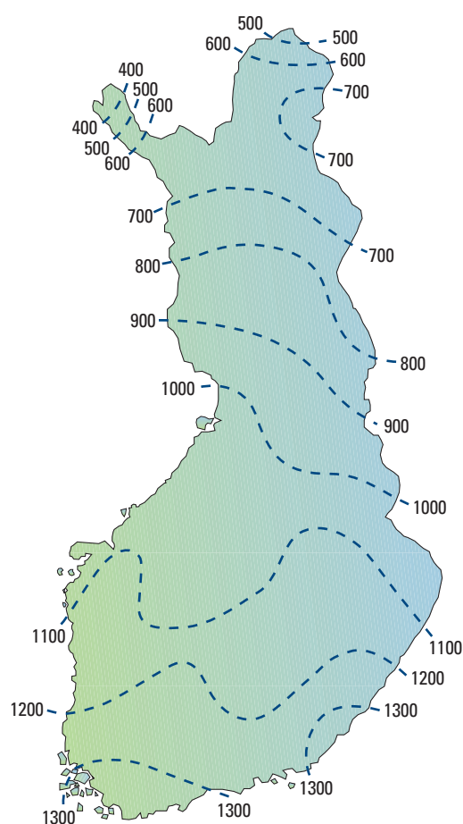
Figure 2-15 Effective temperature sum ( ^{\circ}\text{C} ) in Finland in 1961–90 (Finnish Meteorological Institute, Internet pages)
