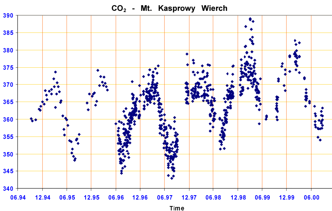
Figure 8.1. Record of carbon dioxide concentration change [ppm] on Mt. Kasprowy Wierch in the period of 1994-2000
