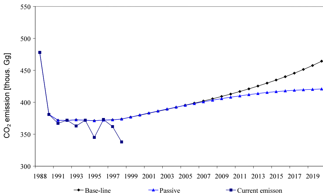
Fig. 5.1. Potential changes of CO 2 emission in Poland according to the two scenarios: the base-line scenario and the passive scenario and the current emission estimated
