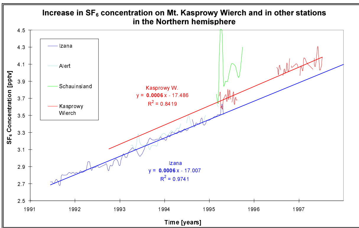
Figure 8.3. SF 6 concentration changes measured on measuring stations in the period of 1991-1997. Results obtained on Kasprowy Wierch are marked in red colour. Regression straight lines are drawn-up for Kasprowy Wierch (Poland) and Izana (Canary Islands) stations
