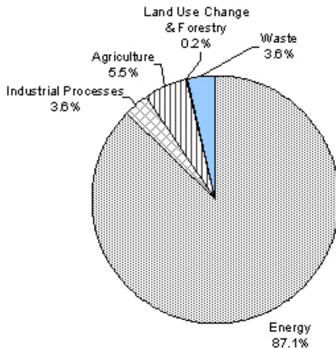
Figure 3.5. The share of greenhouse gas emissions by source category in 1988 Source: MS
