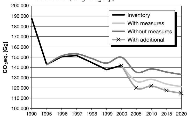
Fig. 5-1 GHG emission projections – reference scenario (kt of CO 2 eq.)
