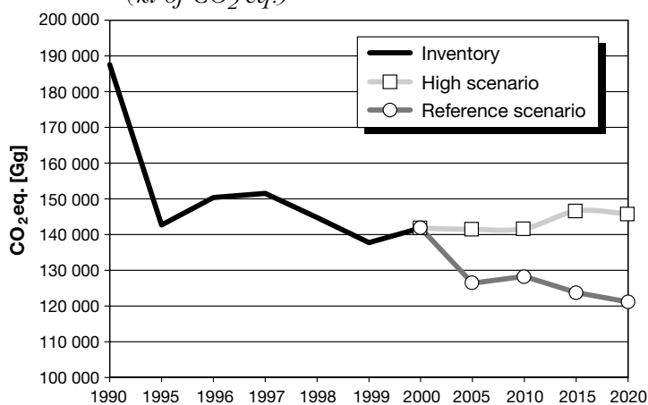
Fig. 5-3 GHG emission projections – high and reference scenarios with measures (kt of CO 2 eq.)
