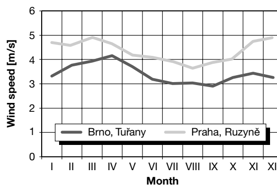
Fig. 2-6 Annual course of mean wind speed in 1961–1990
