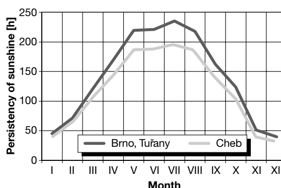
Fig. 2-5 Annual course of sunshine duration in 1961–1990
